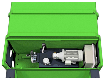
fest eingebautes Hydraulikaggregat fix mounted hydraulic aggregate
