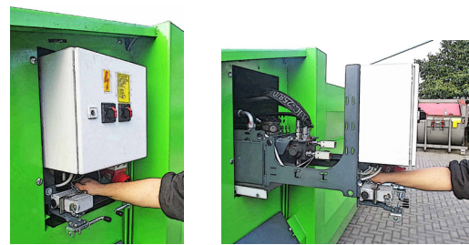
herausziehbares Hydraulikaggregat extractable hydraulic aggregate
